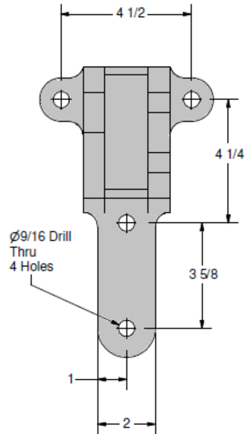
Right Hanger Bracket
