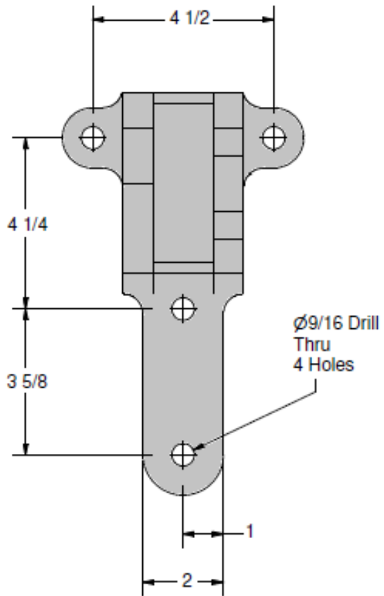
Left Hanger Bracket
